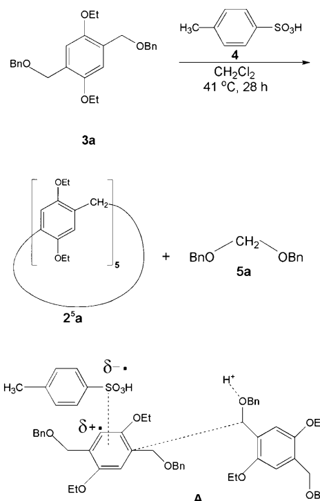
Scheme 2. Generation of ethyl-substituted pillar[5]arene 2 5a .
