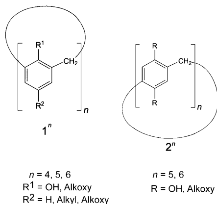
Scheme 1. Calixarenes 1 n and their para -bridged analogues 2 n , which are called pillararenes.
